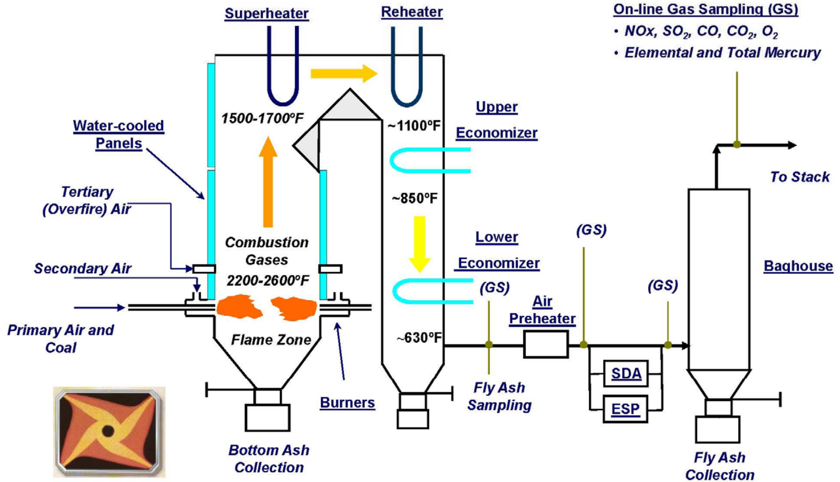
Tangential Firing Burner Configuration
